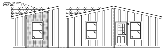
OPTIONAL UPGRADED HITCH END ELEVATION
